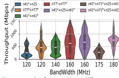
Figure 5: CA boosts Tput. The contour shows data distribution.
