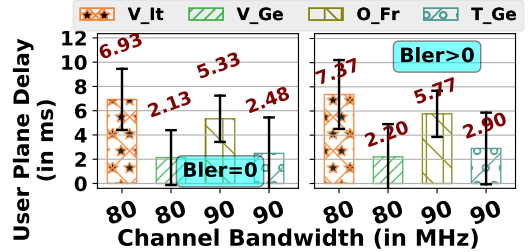
Figure 10: 5G PHY User Plane Latency for different BLER.
