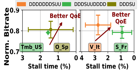
Figure 22: Impact of Frame Structure on QoE, Left subgraph operators use 100 MHz, right subgraph use 80 MHz.
