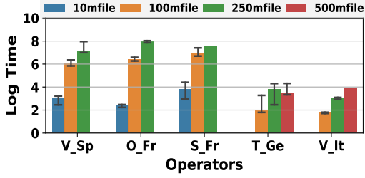
Figure 17: File Download Time.
