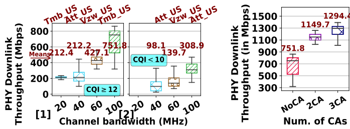
(a) US Operators: when no CA is employed. (b) Benefits of CA with TMB_US.
