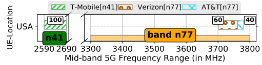
Figure 28: [US] 5G channel bandwidth.
