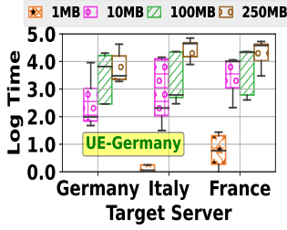
Figure 24: Impact of Server Placement on Download Time.
