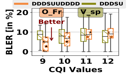
Figure 13: [CB=90 MHz] BLER vs. CQI.
