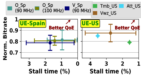
Figure 20: Impact of Channel bandwidth on QoE.
