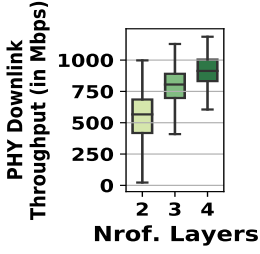
Figure 7: Impact of MIMO on DL Tput.
