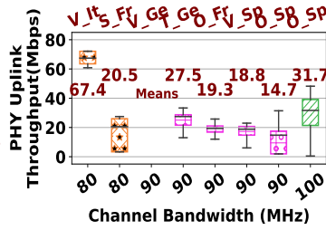
(b) Europe CQI < 10.
