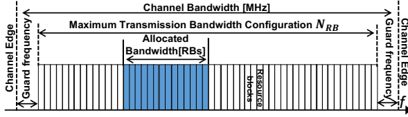
Figure 26: Relationship between channel bandwidth and N_{RB} .
