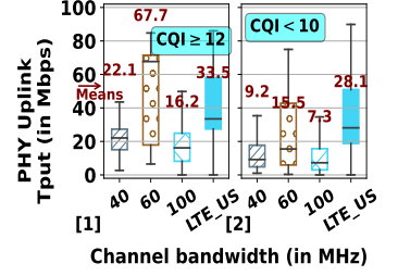
Figure 9: Phy Uplink Throughput US.
