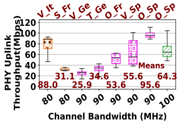
(a) Europe CQI ≥ 12.
