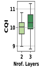
Figure 6: Channel condition and MIMO layers.
