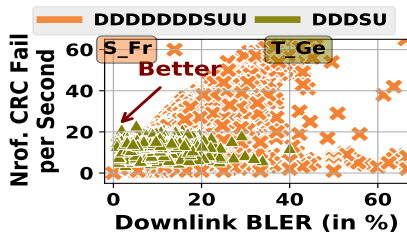
Figure 16: Frame impact on BLER.
