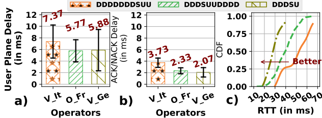
Figure 14: Comparing a) user plane delay, b) ACK/NACK delay, and c) RTT with DDDDDDDSUU, DDDSUUUUUUU and DDDSU.
