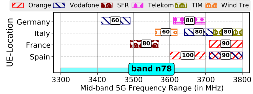
Figure 27: [Europe] 5G Mid-band 5G channel bandwidth.
