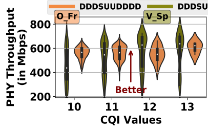
Figure 11: [CB=90 MHz] DL Throughput vs CQI.
