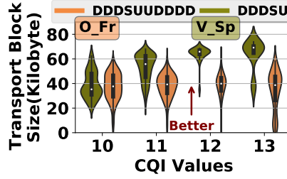
Figure 12: [CB=90 MHz] Transport block sizes vs. CQI.
