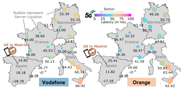
Figure 1: Round-trip-time measurements from UE in Madrid, Spain to Ookla speedtest servers located in four European countries. 5G carriers & mid-band channels: Vodafone Spain with 90 MHz (left) vs. Orange Spain with 100 MHz (right).
