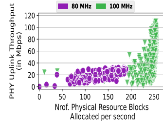
Figure 32: PHY UL Throughput vs. N\_RBs .
