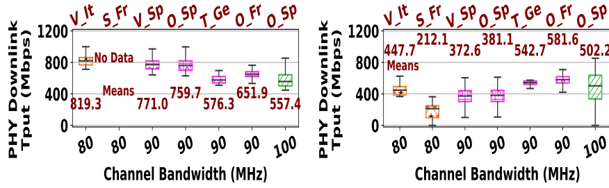
(a) Under Good Channel Conditions: CQI \geq 12 . (b) Under Poor Channel Conditions: CQI < 10 .
