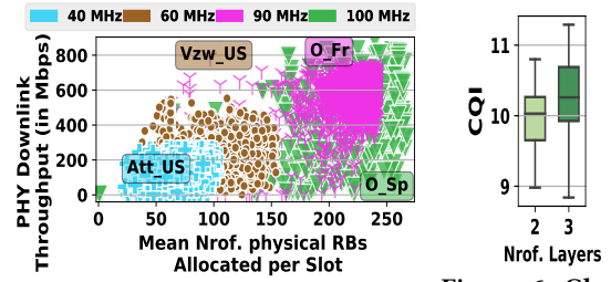
Figure 6: Channel condition and MIMO layers.
