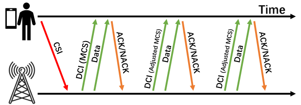
Figure 29: CSI Feedback and DCI scheduling for downlink.
