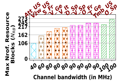
Figure 3: Max Resource Block (RB) Allocation per operator and channel bandwidth.
