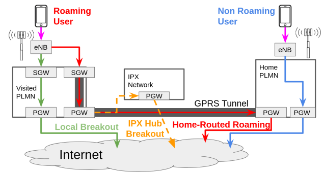
Fig. 2. Mobile network roaming and non-roaming user paths.
