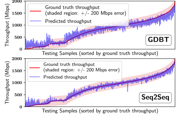
Figure 16: Regression plots for Seq2Seq and GDBT using L+M+C feature groups on Global dataset.
