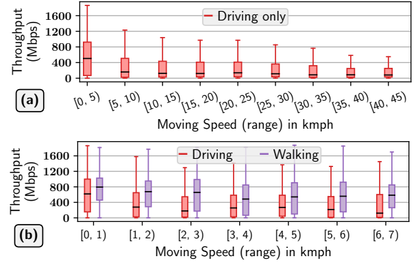
Figure 14: Impact of Mobility Speed on 5G throughput.
