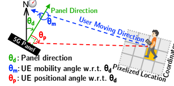
Figure 5: {Panel, Positional, Moving} Angles.
