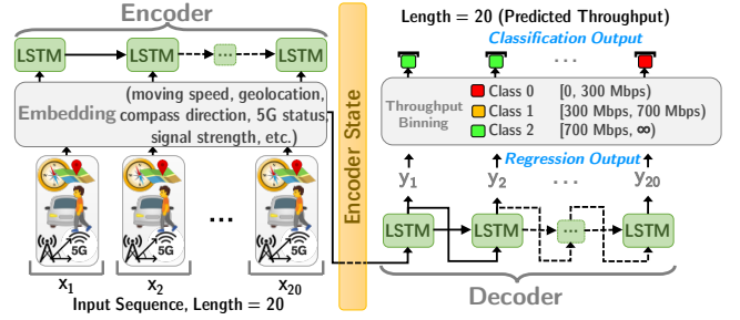
Figure 15: Seq2Seq w/ Encoder-Decoder Architecture.
